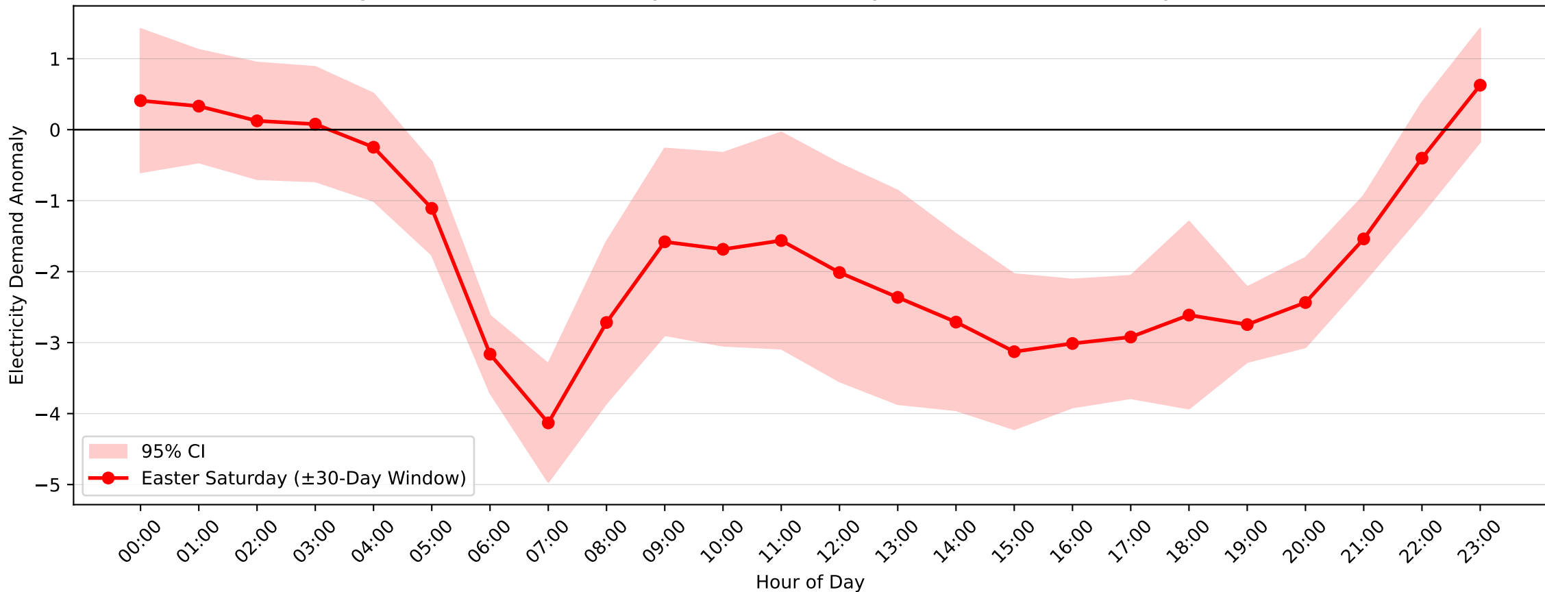
Kogarah Demand Anomaly: Easter Saturday (2004-2017, \pm 30 -Day Window)
